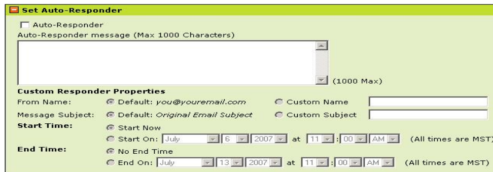
Fig. 3.7 - Auto-Responder Properties.
